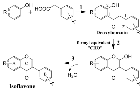
Scheme 1. Synthesis of daidzin analogues.
